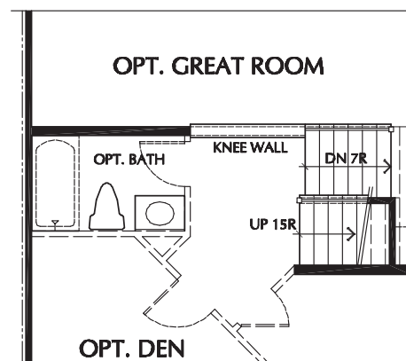
PARTIAL LOWER LEVEL WITH OPTIONAL FULL BATH
